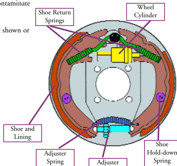
Duo-Servo Cylinder
